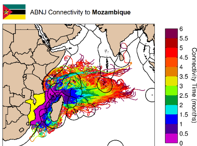
The time, in months, that it takes for ocean surface waters originated in the ABNJ to reach the coastal zone of the Republic of Mozambique. The colour of the trajectories indicate the time in months for the surface waters to be advected to the coastal zone, termed on the colour bar as the connectivity time.
